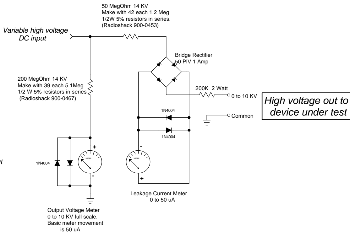
High voltage leakage detector and metering circuit
